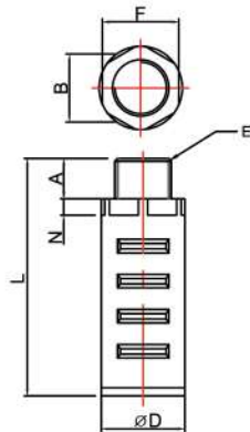
BPS series Stainless steel wire silencer with plastic housing
