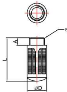
PS series Plastic silencer
